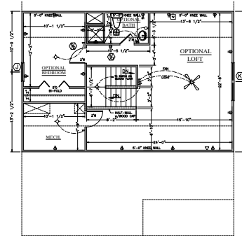
OPTIONAL LOFT w/ BEDROOM & BATH AREA: 752 sf 1/8" = 1'-0"
