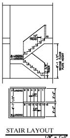
STAIR LAYOUT 1/8" = 1'-0"
